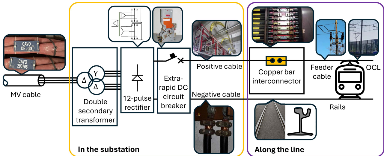
Fig. 2. Building blocks of the Turin UTES.
