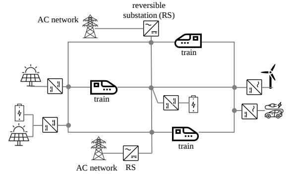
Fig. 1. DC-power SETS scheme.
